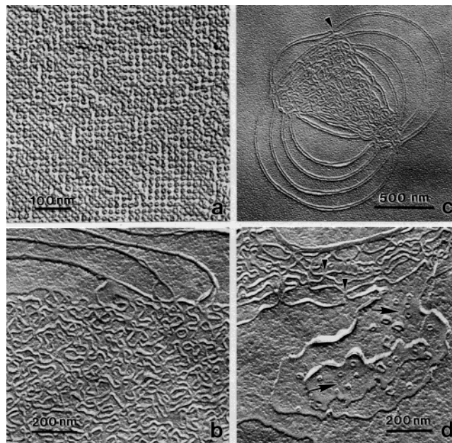
Figure 4. FFEM of compound 1 after gentle hydration at 94 wt % (a) and 97 wt % (b–d) water content. (a) Projection with a regular pattern of a cubic 3D structure. Repeat distance of about 18 nm of the orthogonally arranged elements (tunnels). (b) Projection of a spongelike 3D structure after storage over 10 days at room temperature. A transition to tightly coupled lamellae is visible. (c) Structural transition from a spongelike nucleus to peripheral two-by-two arranged lamellae. Interconnection at the end of two lamellar loops (arrowhead). (d) Tangentially running fracture plane near the surface of lamellar faces with a number of tunnel-like structures (arrows). They may be descended from interconnections of the sponge structure (arrowheads).
