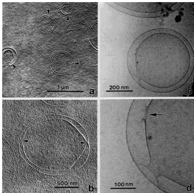
Figure 3. Freeze-fracture electron microscopy (FFEM; a, b) and Cryo-TEM (c, d) of glycolipid 1 after hydration by intensive stirring in excess water (99 wt %). (a) Vesicles with two-by-two lamellar arrangement showing an interconnection (arrowheads) between the two envelopes. (b) Vesicle with two-by-two lamellar arrangement showing two tunnel-like interconnections (arrowheads). (c) Cryo-TEM of vesicular two-by-two lamellar arrangements. The inside vesicle looks like an invagination of the outer envelope. (d) At higher magnification, a second interconnection of the two membranes is clearly visible (arrow).
